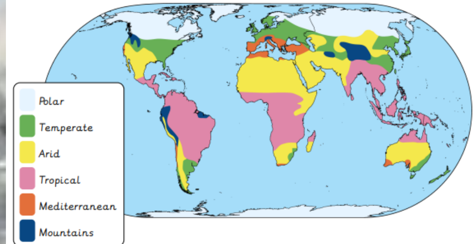
Climate zone map
